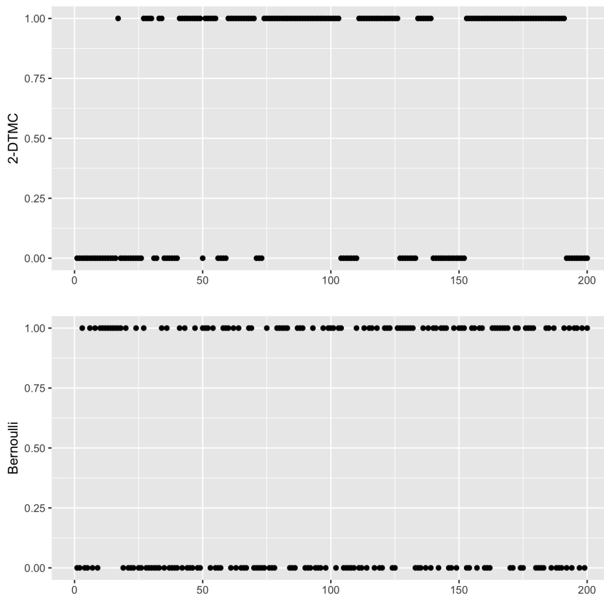
Figure 1: Sample paths from the 2-DTMC and Bernoulli process generated by the supplied helper.
