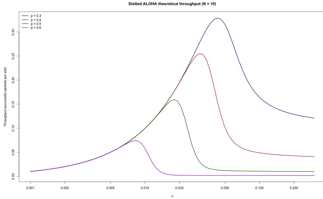
Figure 2: Theoretical slotted-ALOHA throughput for N = 10 and the four requested values of p .
