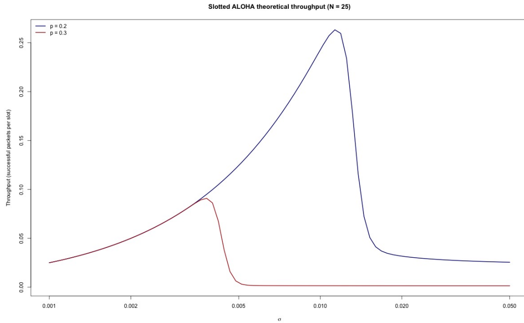
Figure 3: Theoretical slotted-ALOHA throughput for N = 25 and the two requested values of p .
